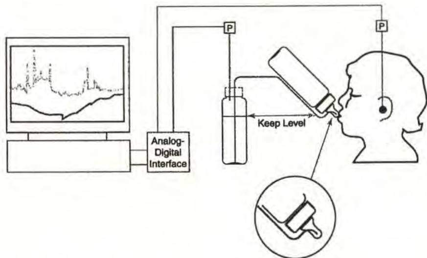
Fig. 1. Equipment used to digitally record simultaneous ear and bottle pressure measurements.
