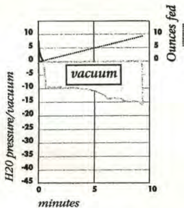
Fig. 6. Pressure graph showing a slower induction of negative pressure occurring in an under-vented bottle, which became significant over time.
