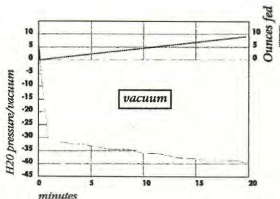
Fig. 4. Pressure graph showing the rapid induction of negative pressure occurring within a non-vented bottle, which became very significant.
